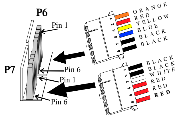
Power Supply Connectors
